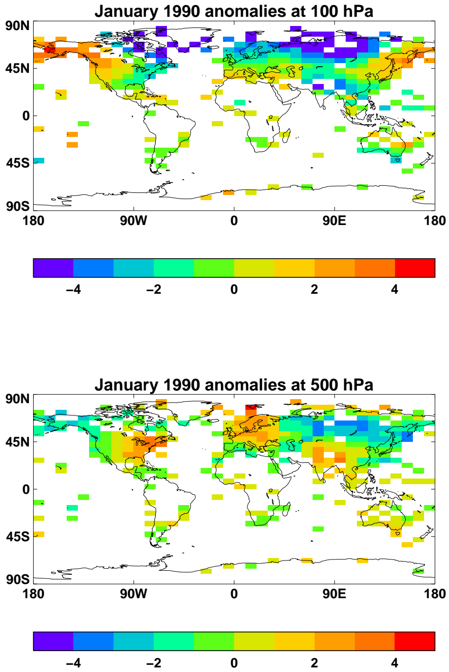
Figure 4: As Figure 3 but for January 1990
