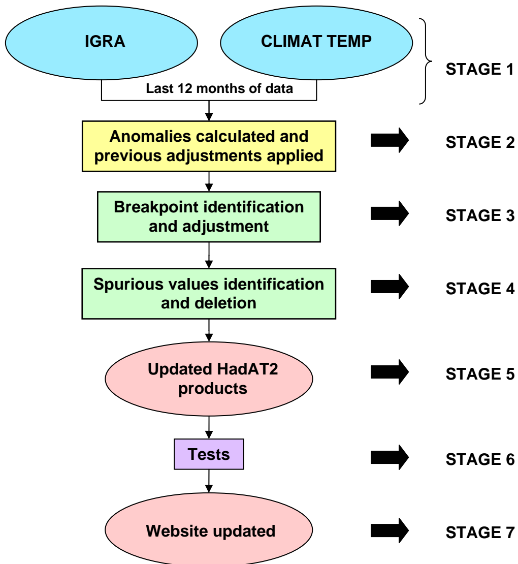
Figure 1: Schematic of the HadAT2 monthly update process
