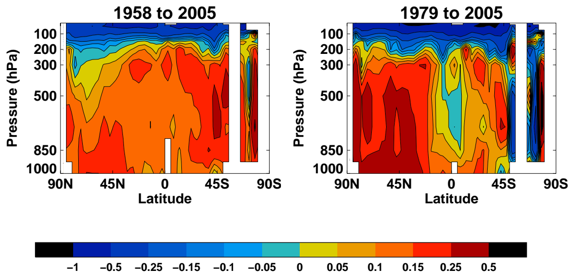
Figure 7: Linear trends in zonal mean temperature (K/decade) in HadAT2 for 1958-2005 and 1979-2005. 1000hPa data are from HadCRUT2v subsampled to the time-varying HadAT2 500hPa availability
