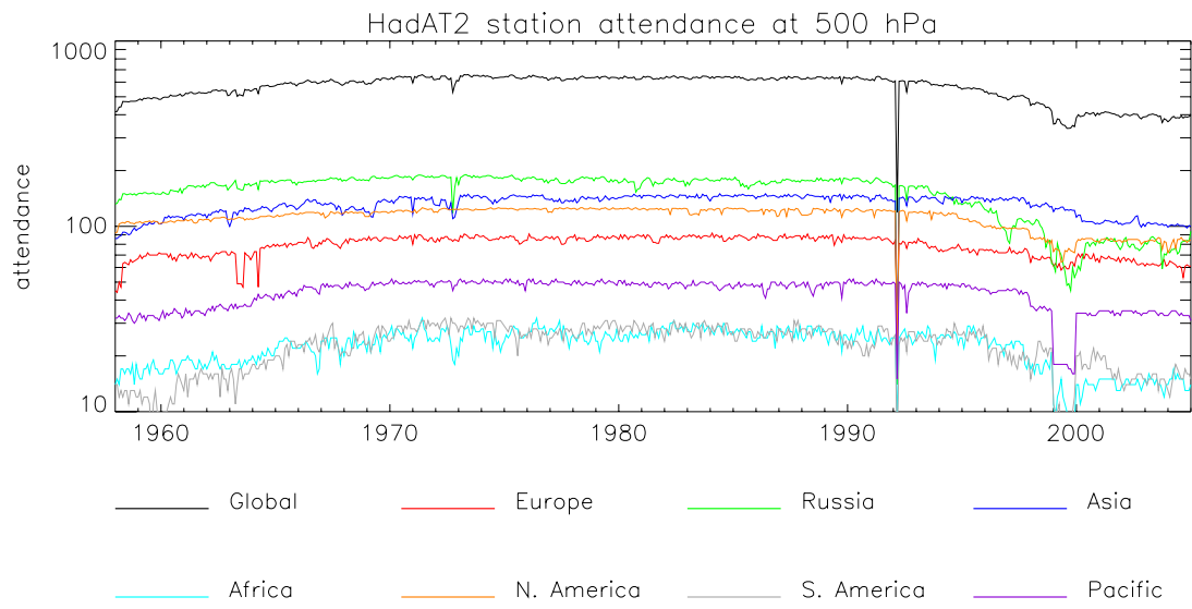
Figure 5: Plot of HadAT2 global and regional station attendance at 500hPa. Note the logarithmic y-axis.
