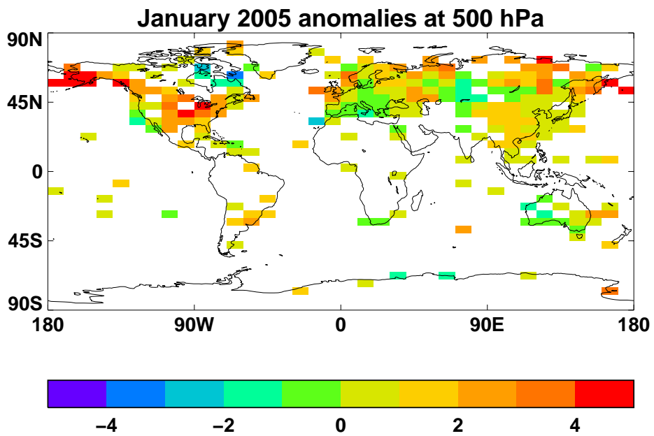
Figure 3: Plots of HadAT2 gridded monthly temperature anomalies (K) for January 2005 at 100hPa and 500hPa.
