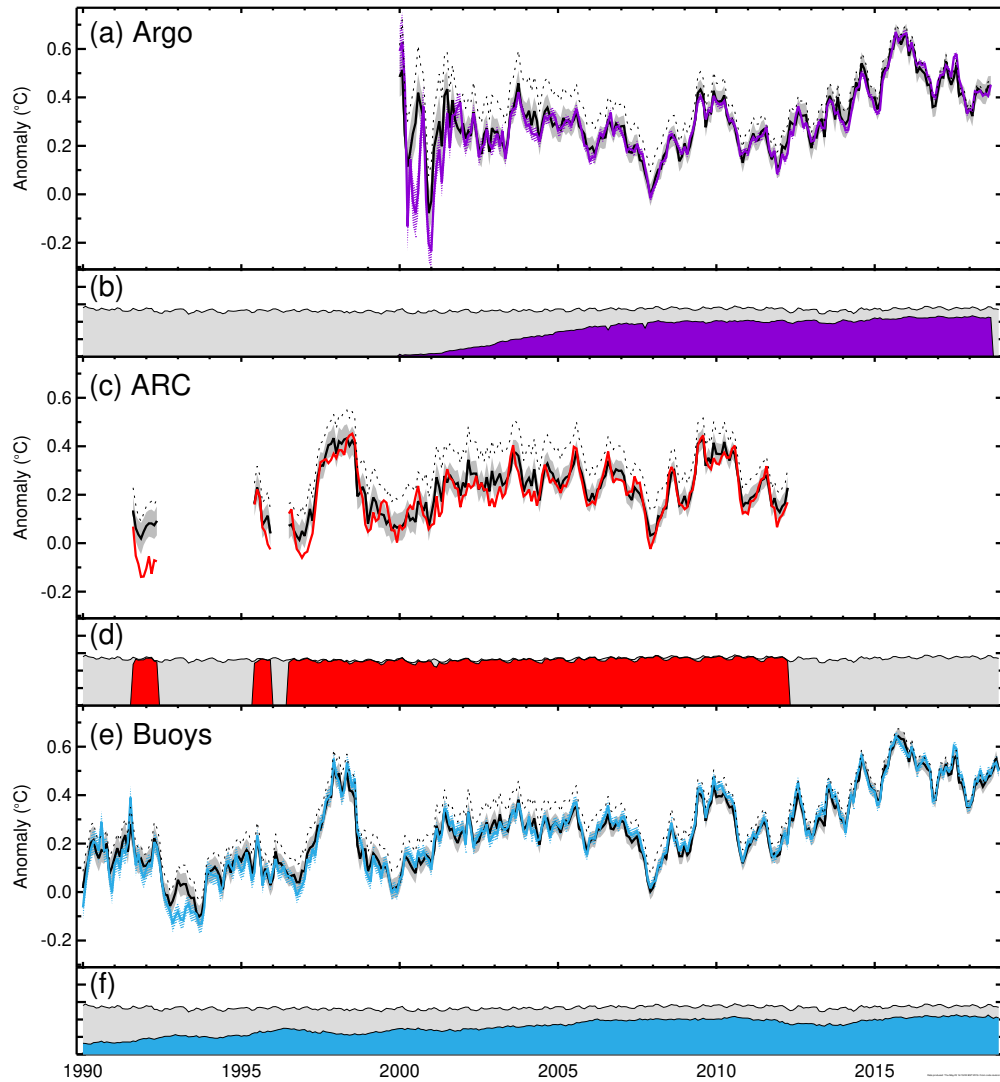
Figure 6: From [13]. Comparison to instrumentally homogeneous data sets. (a) global average SST anomalies from Argo (purple) and HadSST.4.0.0.0 (black and grey shading). The dotted line shows a global average calculated from unadjusted data. All comparisons are colocated. (b) coverage of HadSST.4.0.0.0 (grey) and coverage of the Argo data (purple). (c) and (d) as for (a) and (b) but for ARC data. (e) and (f) as for (a) and (b) but for drifting buoy data.
