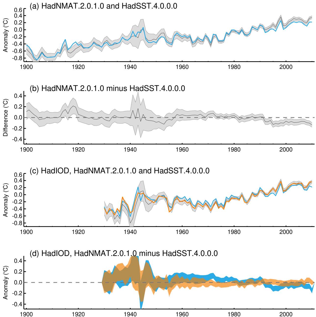
Figure 5: From [13]. (a) Collocated global annual average NMAT anomalies ( ^{\circ}\text{C} ) 1900-2010 offset by 0.15^{\circ}\text{C} (blue, relative to 1961-1990) and global annual average SST anomalies from HadSST.4.0.0.0 (black is central estimate and grey shading indicates 95% uncertainty range). (b) Offset NMAT anomalies minus SST anomalies with combined 95% uncertainty range (taking into account the bias errors from the HadSST.4.0.0.0 ensemble, and measurement and sampling errors in the SST). The dashed line indicates zero difference. (c) Collocated global annual average offset NMAT anomalies (blue), global annual average near-surface water temperature from HadIOD excluding Argo (orange) and SST (black is central estimate and grey shading again indicates 95% uncertainty range). (d) Difference between HadIOD and HadSST.4.0.0.0 (orange) and NMAT and HadSST.4.0.0.0 (blue). The shaded area indicates the 95% uncertainty range..
