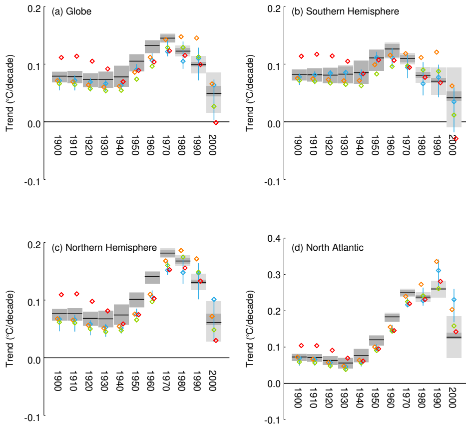
Figure 4: From [13]. Global and regional average SST anomaly trends to 2012. Median trends from HadSST.4.0.0.0 are indicated by a black horizontal line and the grey shading indicates median and 95% uncertainty range including effects from measurement, sampling and bias-adjustment errors. The bias-adjustment uncertainty range is shown in darker grey; ERSSTv5 (blue), the lozenge is the operational version and the vertical line is the 95% ensemble range from the 1000-member ERSSTv4 ensemble); COBE-SST-2 (orange); HadSST.3.1.1.0 (green); and unadjusted SSTs (red).
